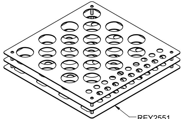
REY2551 VIAL TRAY
